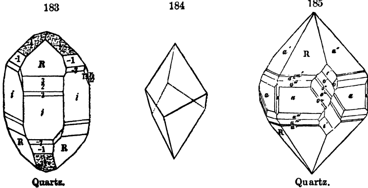
Quartz.
